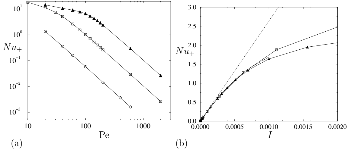
Figure 4: Fully developed Forward Nusselt number for different parameters. Bullet symbols are associated with R = 1.1 , square symbols for R = 2 and black triangular symbols with R = 5 . (a) Versus the Péclet number. (b) Versus the parameter I defined in (9). The leading order asymptotic behavior (20) is shown with dotted lines, while the next order is represented with long dashed lines.
