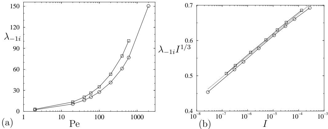
Figure 3: (a) Imaginary part of the first backward eigenvalue \lambda_{-1} versus Pe , for R = 1.1 with circle symbols and R = 1.05 for square symbols with \frac{k^I}{k^{II}} = 1 . (b) Same conventions for \lambda_{-1i} I^{1/3} versus parameter I in semi-logarithmic representation.
