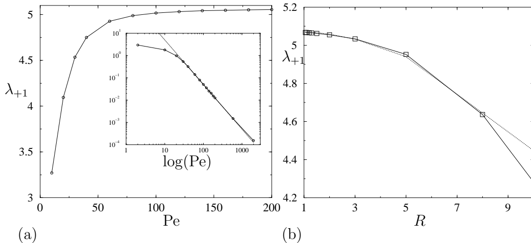
Figure 2: (a) First eigenvalues \lambda_{+1} versus Pe , for R = 2 , \frac{k^I}{k^{II}} = 1 . The inset represents a log-log representation of the difference \lambda_{+1} - \lambda_{+1}^\infty with \lambda_{+1}^\infty = 5.067505 versus the Péclet number; the asymptotic (11) is represented with dotted lines. (b) Same conventions as in figure (a) versus the aspect ratio R for Pe = 200 . Dotted line illustrates the asymptotic (11)
